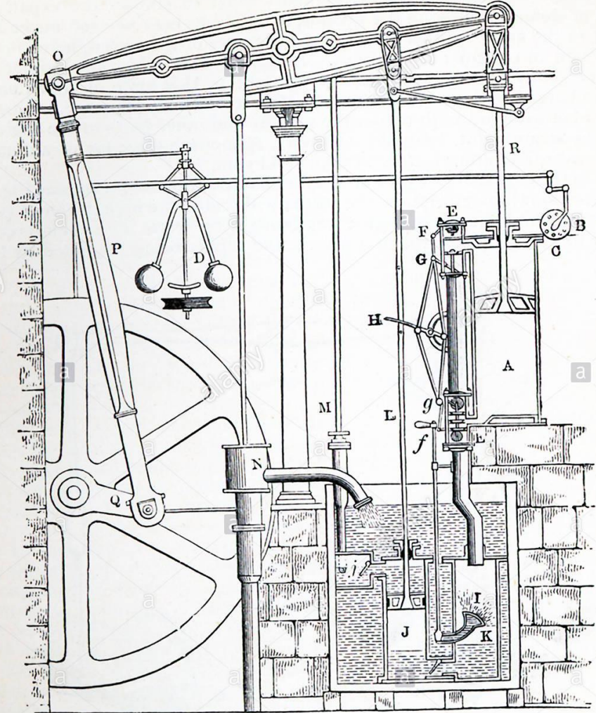
FIG. 3.—Watt's Double-action Steam Engine.
