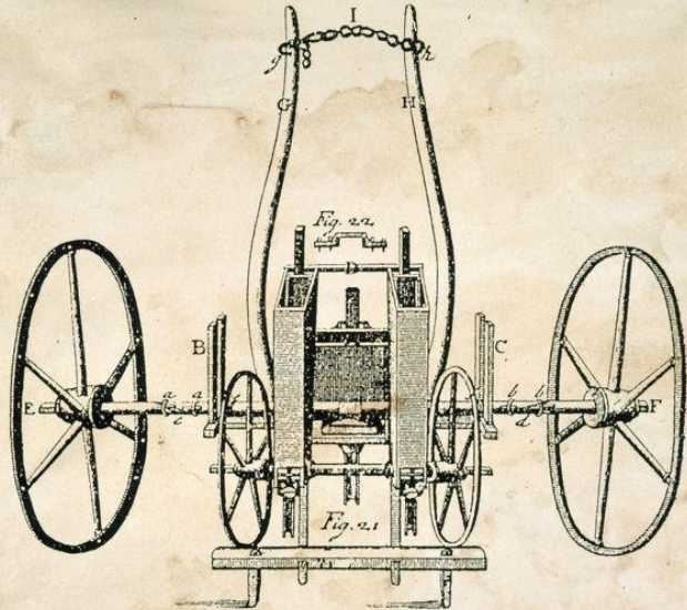
JETHRO TULL'S WHEAT DRILL
